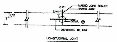
EXPANSION JOINT
